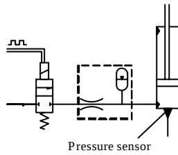
Fig. 8. Inlet Circuit for Control using PWM
